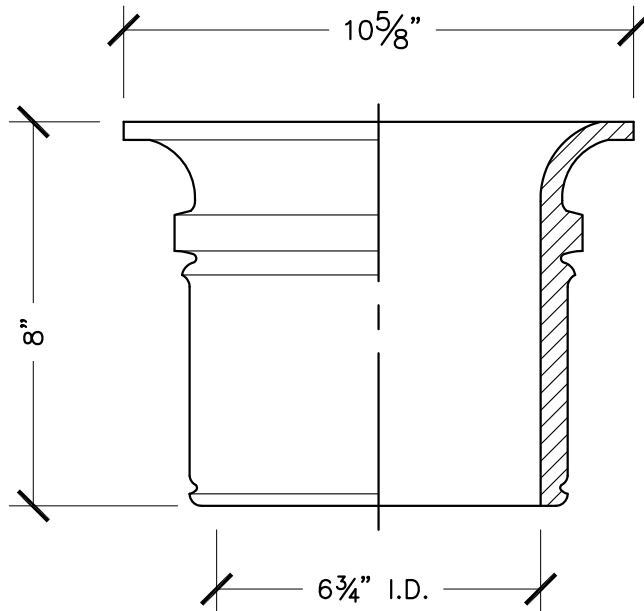
ELEVATION / SECTION
