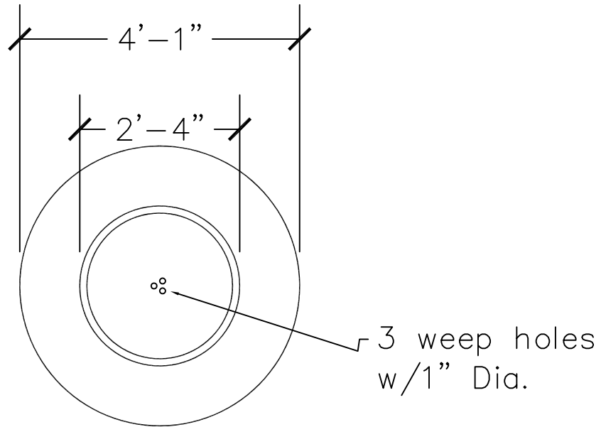
View @ Top
